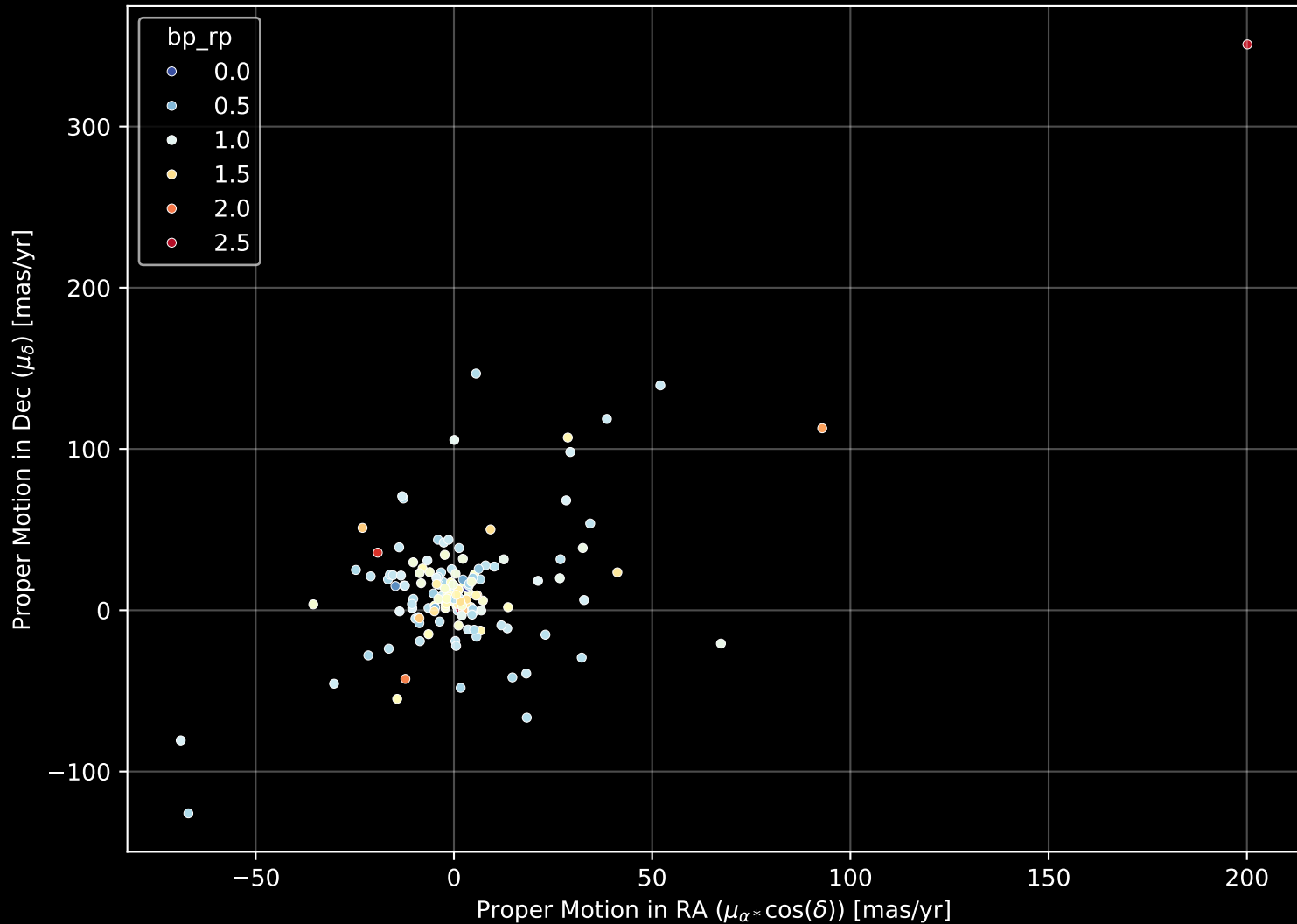
APOGEE DR17 Field: [276-28-O_TESS] Proper Motion Diagram (n= 159)
