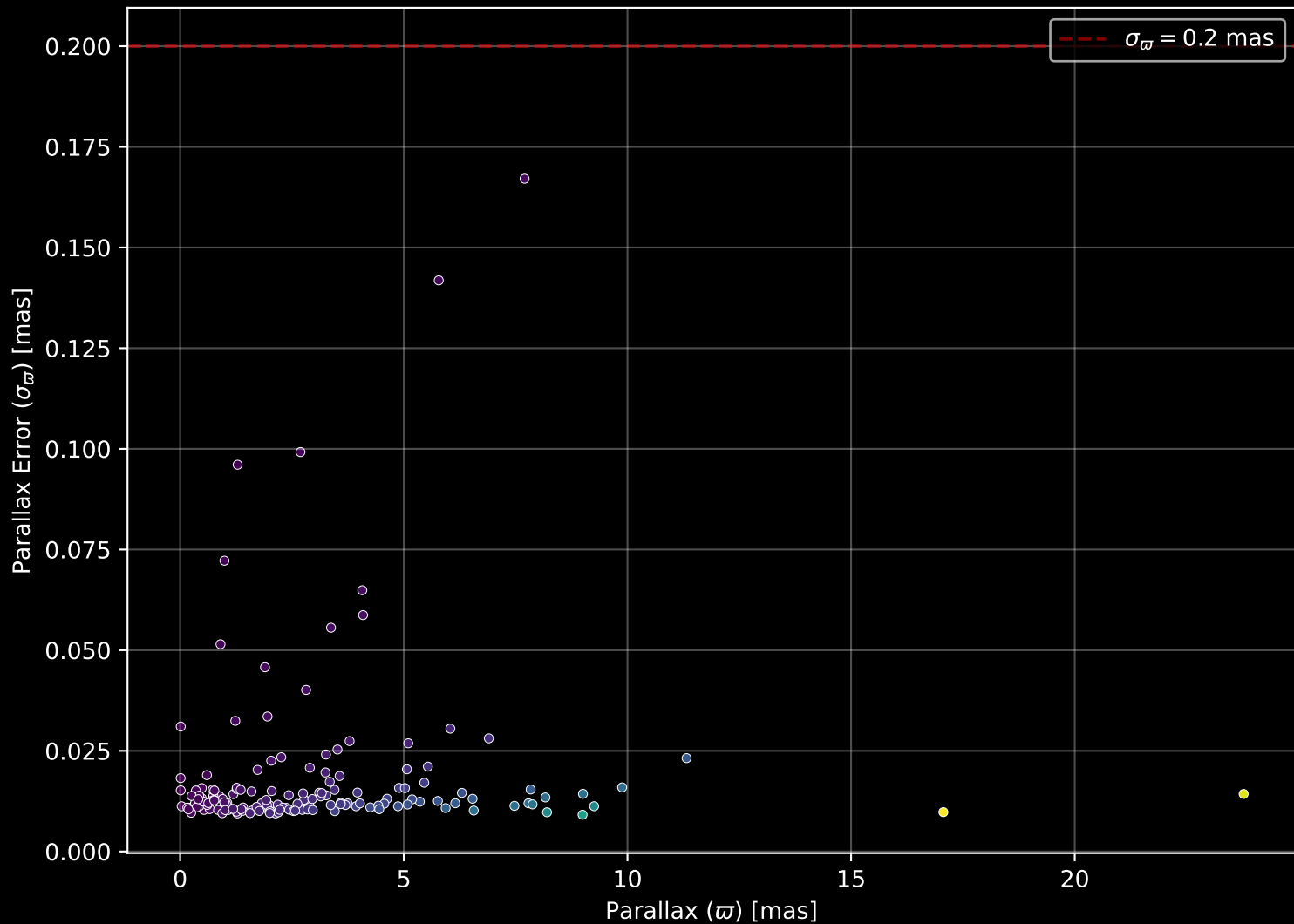
APOGEE DR17 Field: [276-28-O_TESS] Parallax Quality (n= 159)
