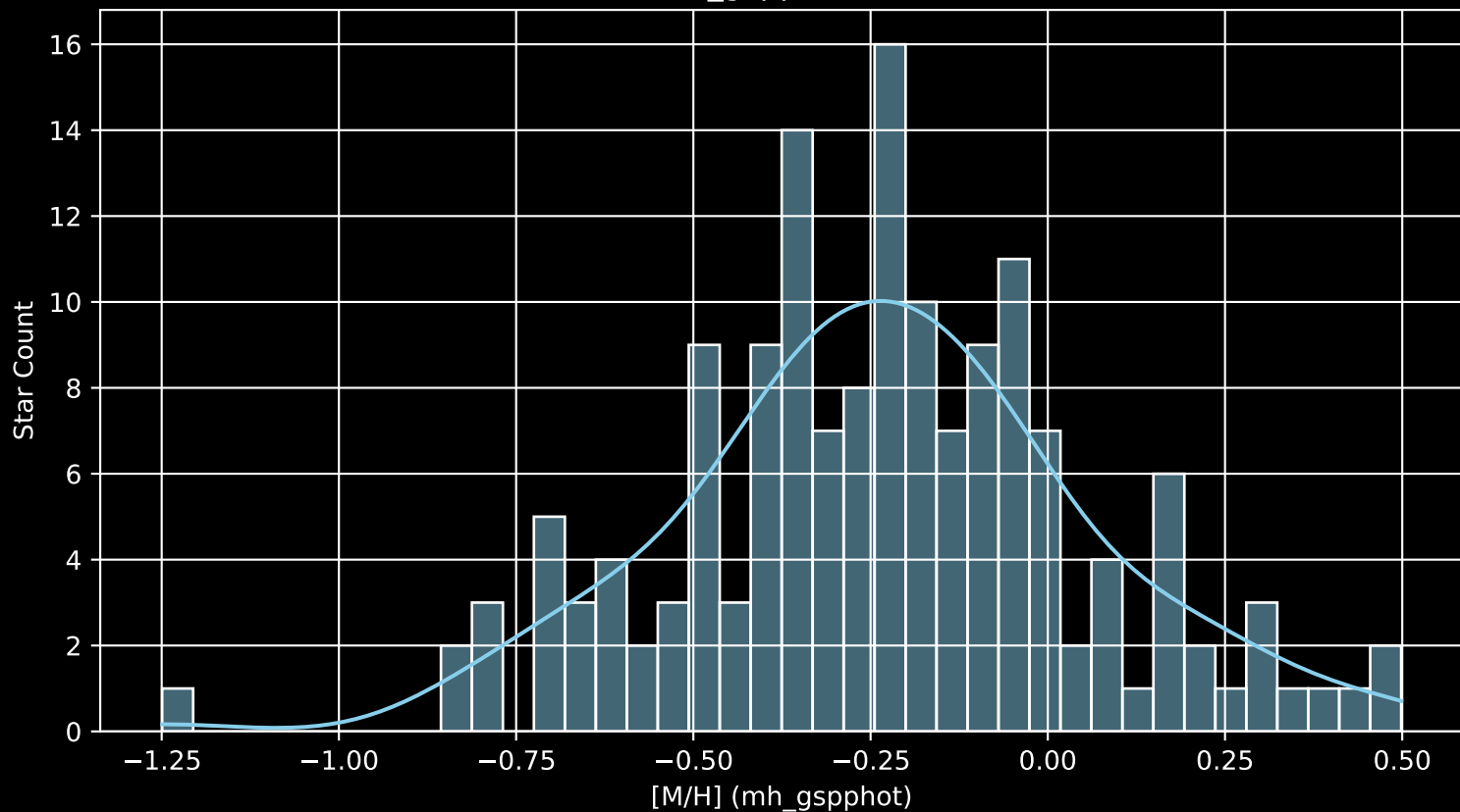
APOGEE DR17 Field: [276-28-O_TESS [M/H] (mh_gspphot) (n= 157)
