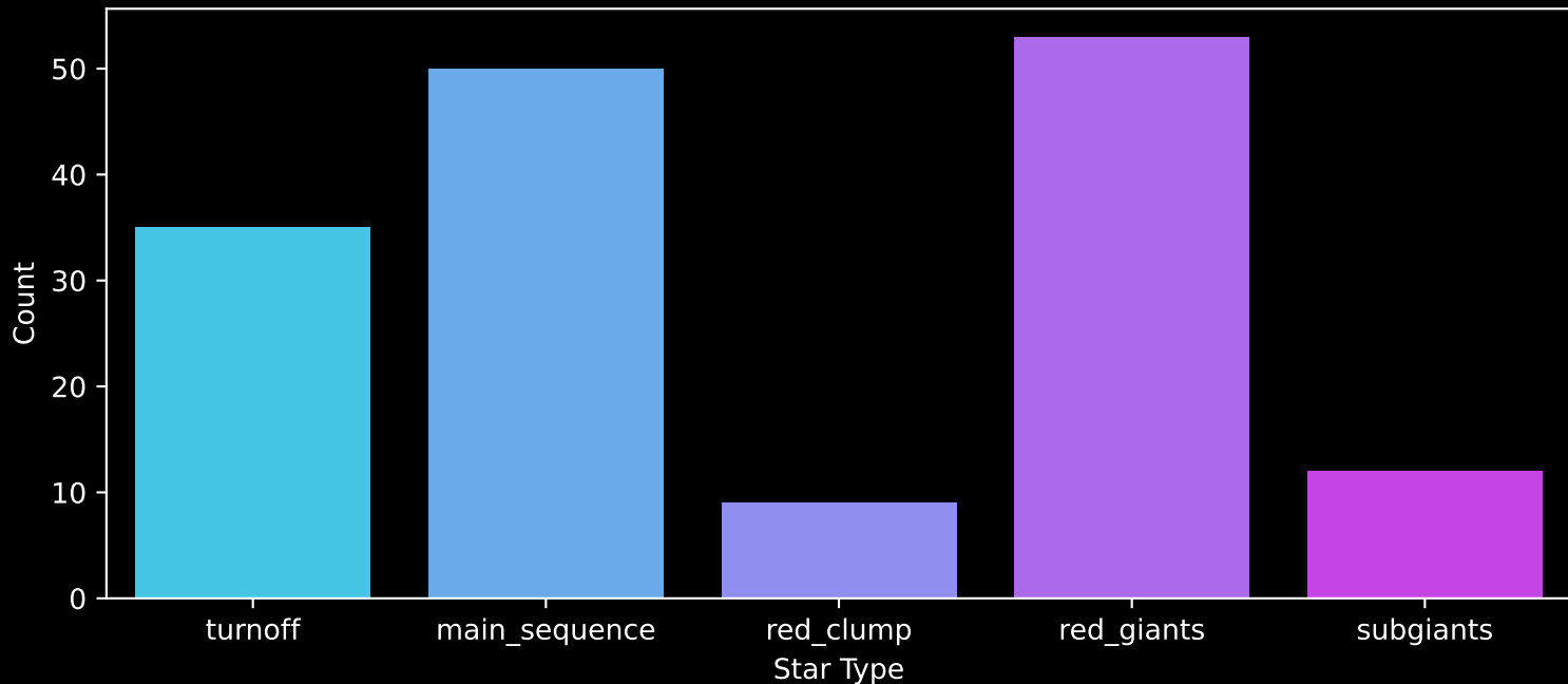
APOGEE DR17 Field: [276-28-O_TESS] Count plot of Star Type
