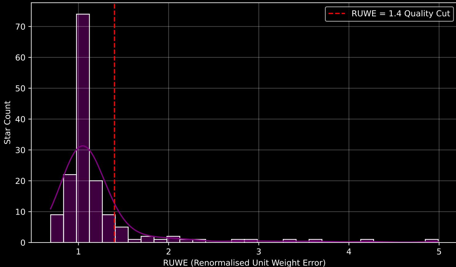
GAPOGEE DR17 Field [276-28-O_TESS] RUWE Distribution (n= 153)
