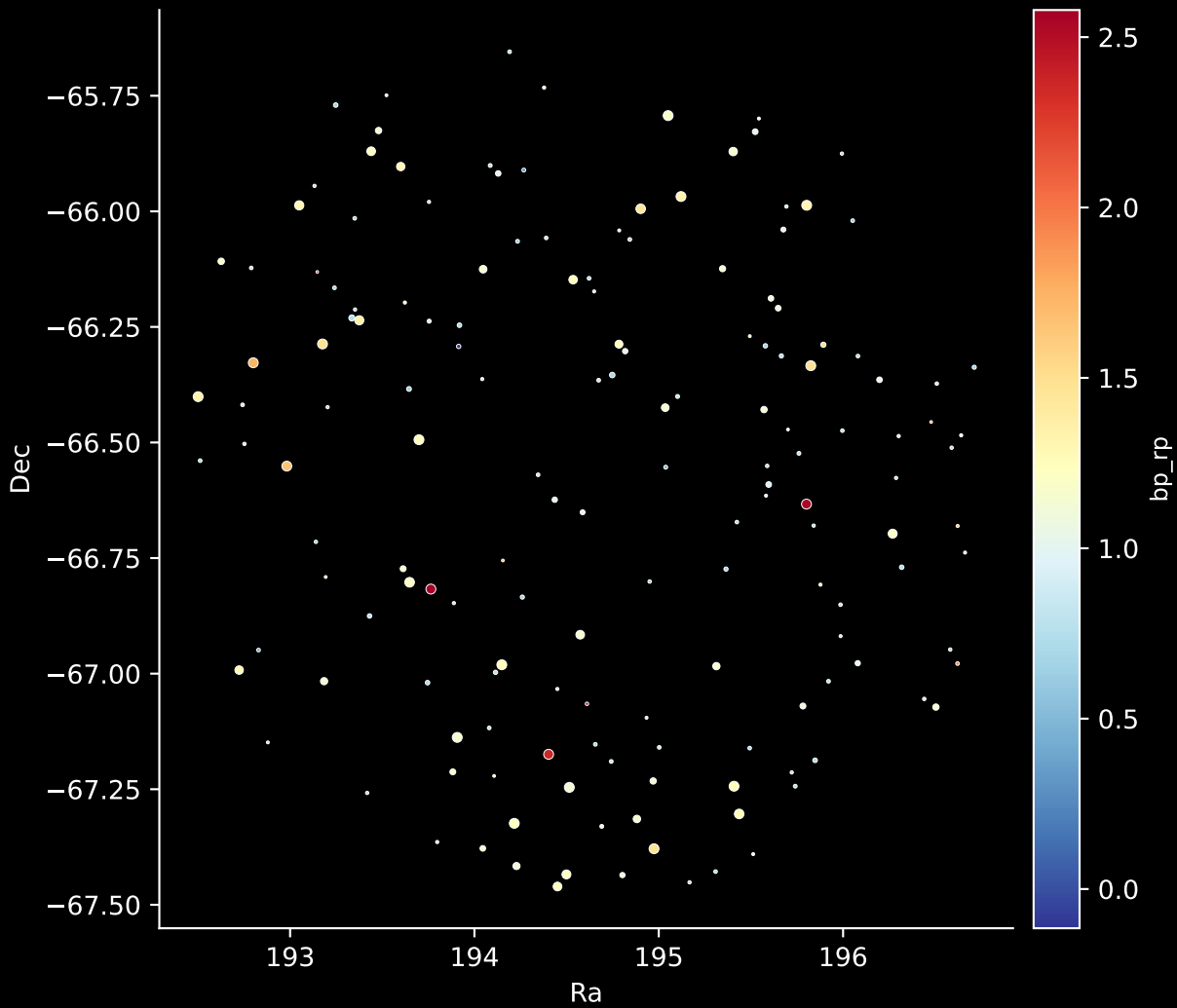
APOGEE DR17 Field: [276-28-O_TESS] Stars: 159
